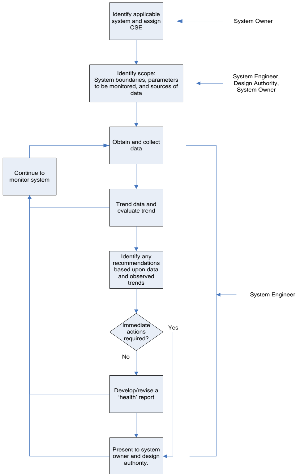
Figure 2 Basic steps of a system health monitoring process.
