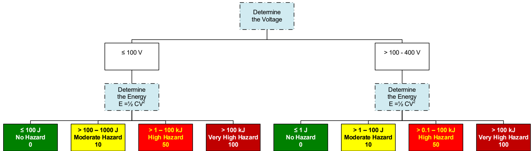
Chart 4. Capacitors, \leq 400 V.
