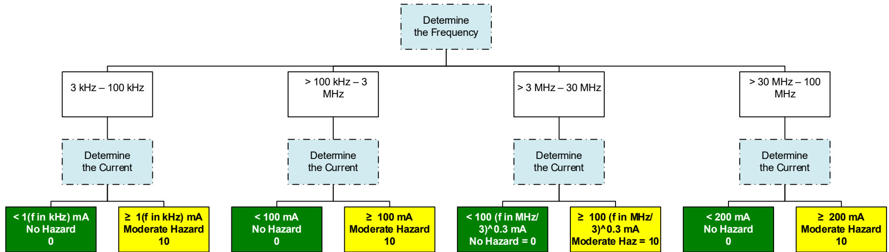
Chart 7. rf circuits, 3 kHz to 100 MHz.
